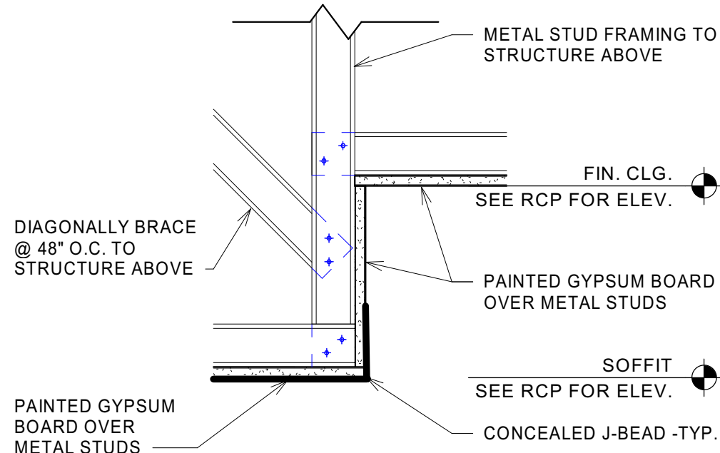
1 Detail TYP CEILING DETAIL
