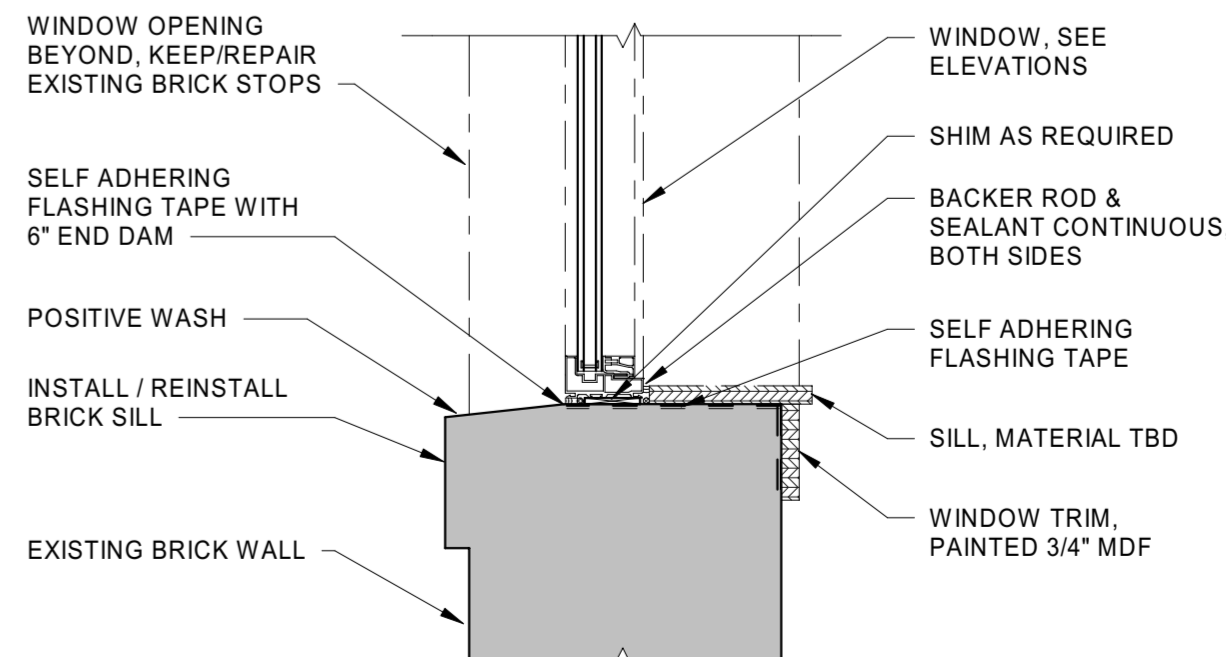
1 Detail Window Sill Existing Brick Opening
