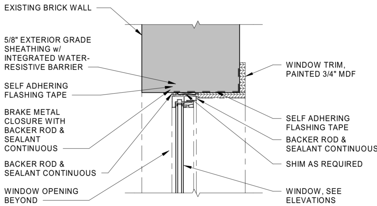
3 Detail Window Head Existing Brick Opening
