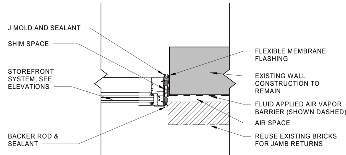
5 Detail AL SF Jamb Existing Brick Opening
