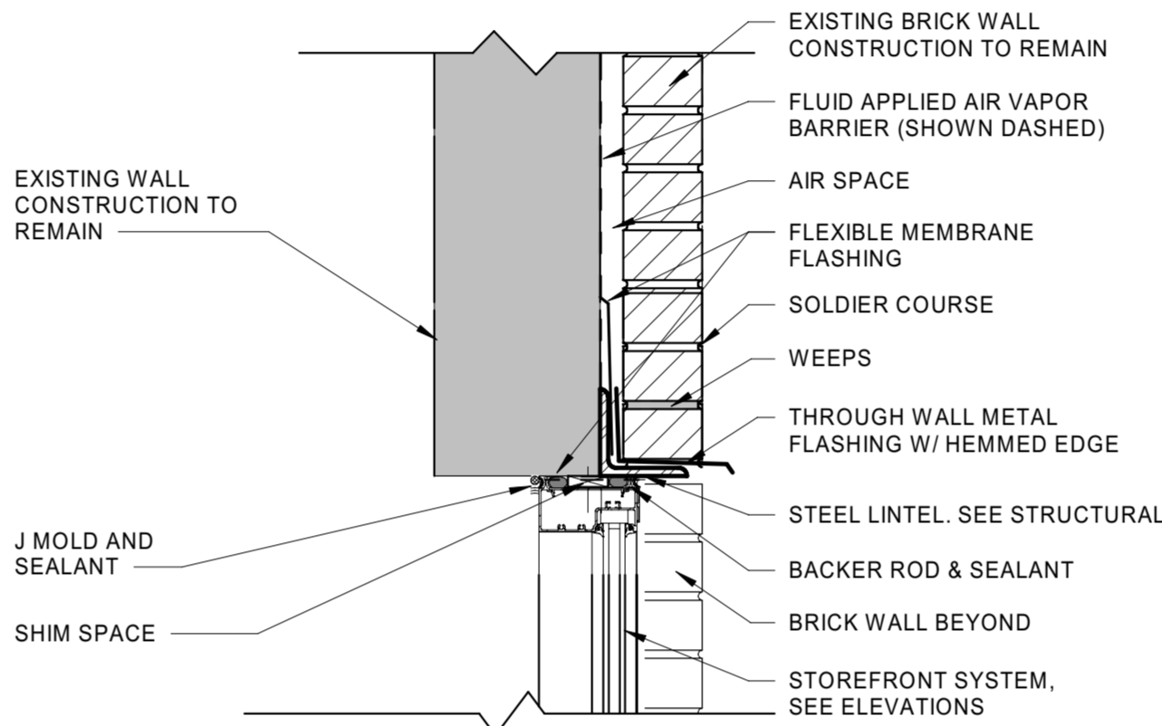
6 Detail AL SF Head Existing Brick Opening
