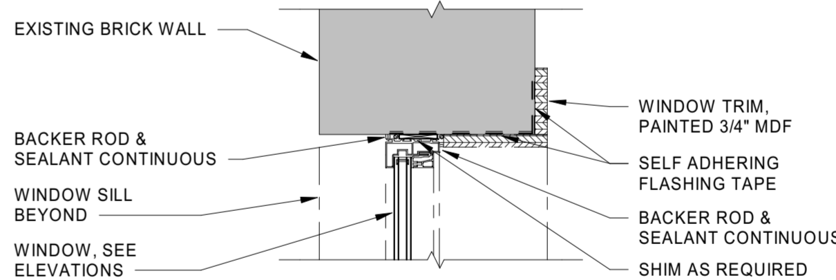
2 Detail Window Jamb Existing Brick Opening
