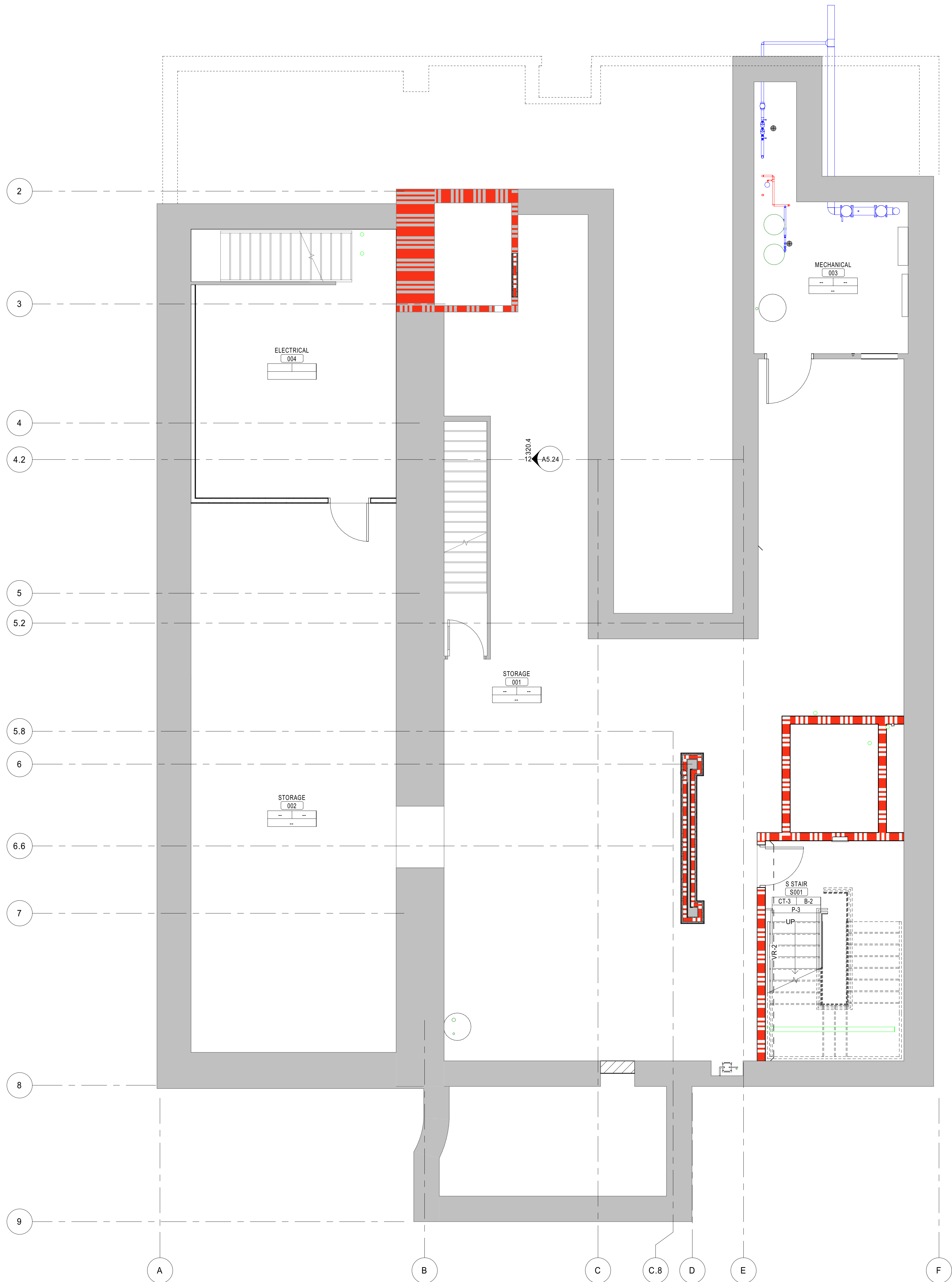
1 Floor Plan Basement, Finish Plan A1.00-F1 1/4" = 1'-0"
