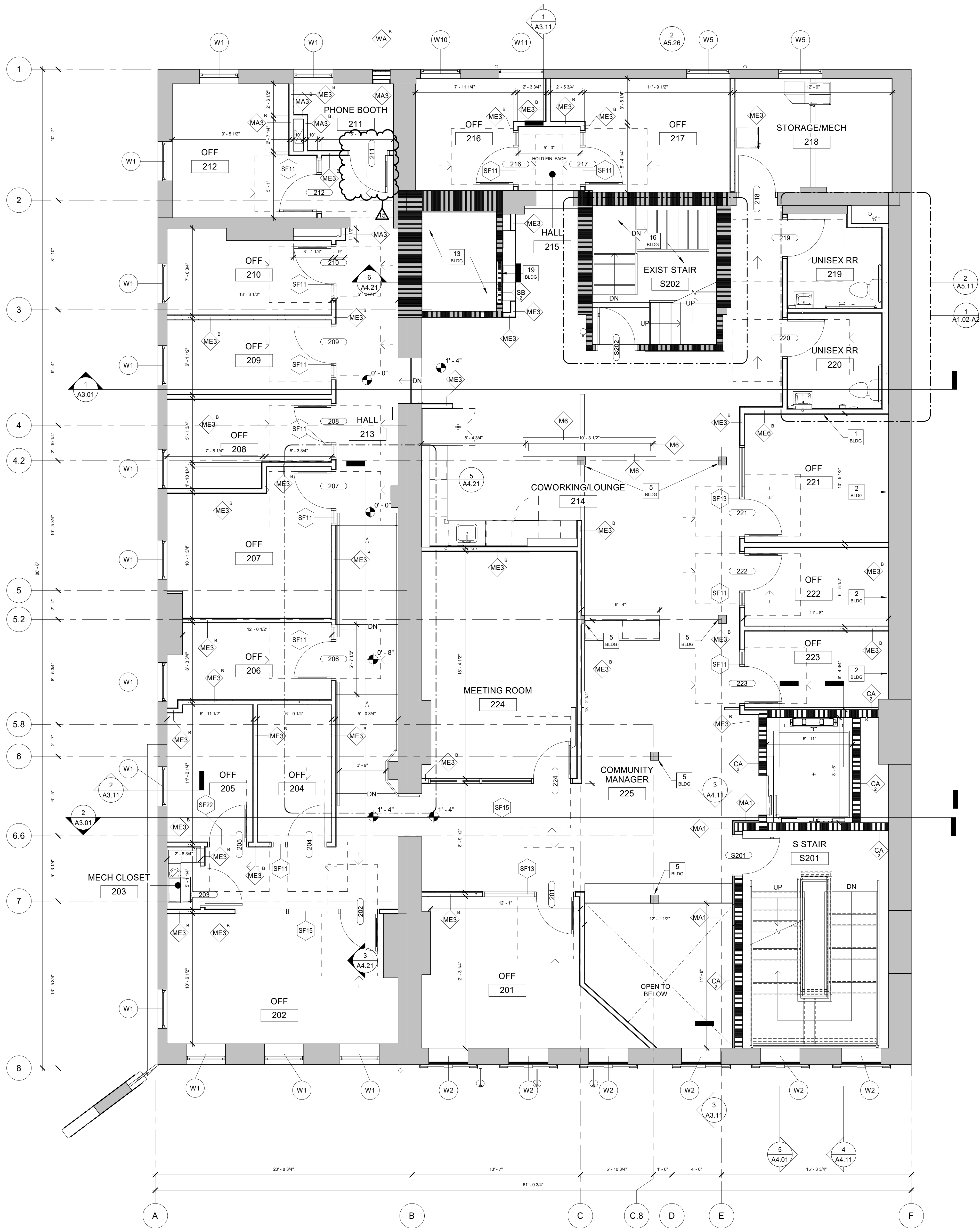
1 Floor Plan 2nd Floor, Plan A1.02-A1 1/4" = 1'-0"
