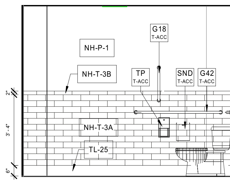
6 Interior Elevation WOMENS RR - 113 - E A5.12 3/8" = 1'-0"
