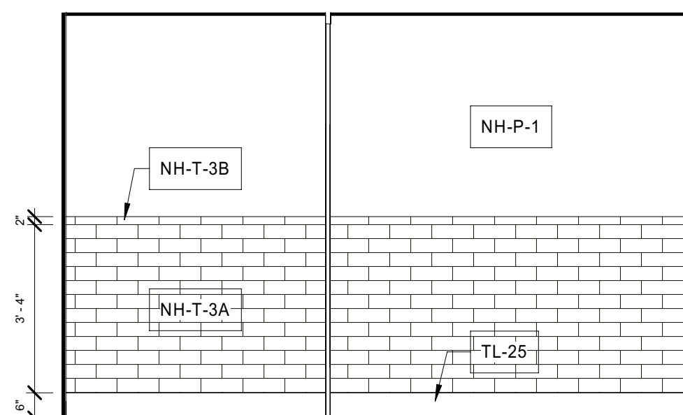
3 Interior Elevation MENS RR - 112 - S A5.12 3/8" = 1'-0"
