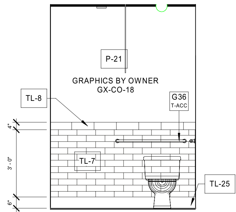
9 Interior Elevation UNISEX RR - 219 - E A5.12 3/8" = 1'-0"
