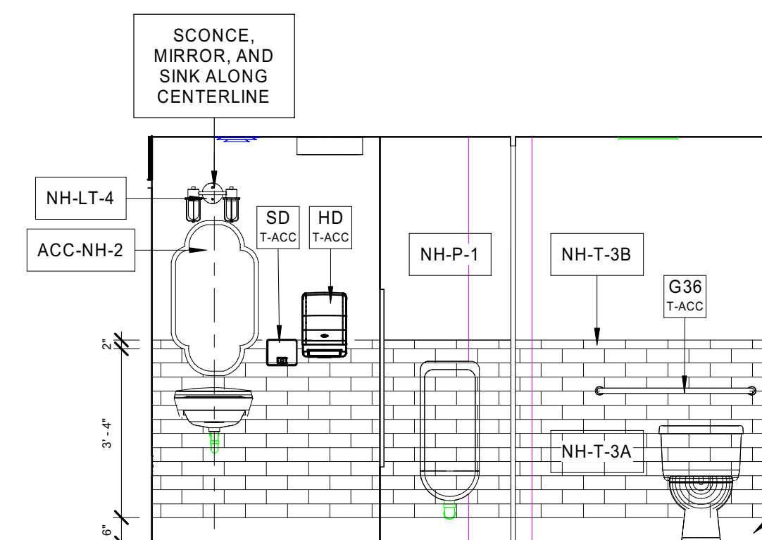
1 Interior Elevation MENS RR - 112 - N A5.12 3/8" = 1'-0"
