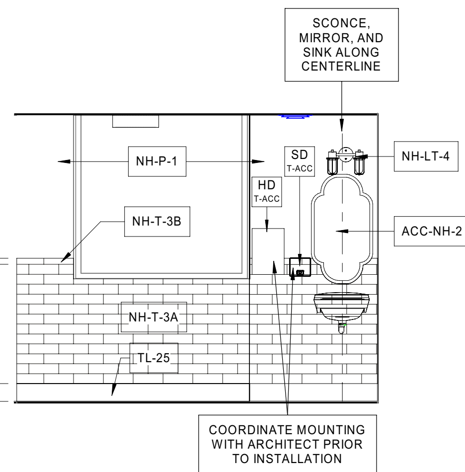
8 Interior Elevation WOMENS RR - 113 - W A5.12 3/8" = 1'-0"
