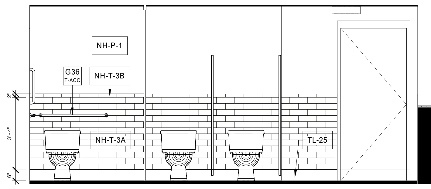
7 Interior Elevation WOMENS RR - 113 - S A5.12 3/8" = 1'-0"
