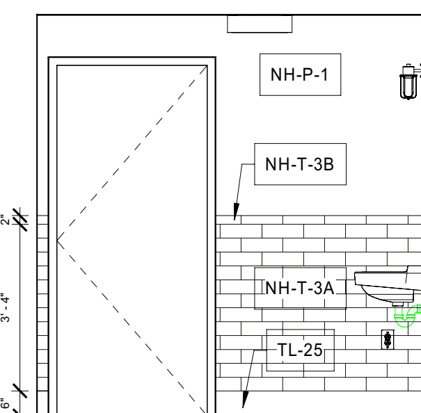
4 Interior Elevation MENS RR - 112 - W A5.12 3/8" = 1'-0"
