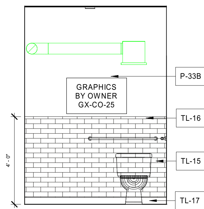
18 Interior Elevation UNISEX RR - 315 - E A5.12 3/8" = 1'-0"
