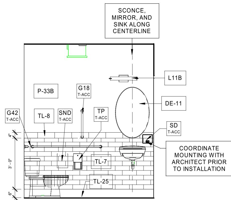
15 Interior Elevation UNISEX RR - 220 - S A5.12 3/8" = 1'-0"
