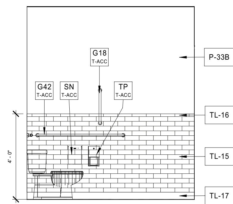
19 Interior Elevation UNISEX RR - 315 - S A5.12 3/8" = 1'-0"
