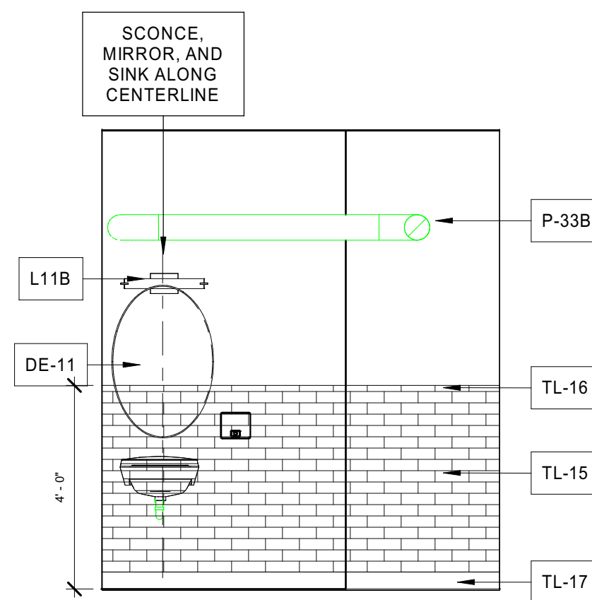
17 Interior Elevation UNISEX RR - 315 - N A5.12 3/8" = 1'-0"
