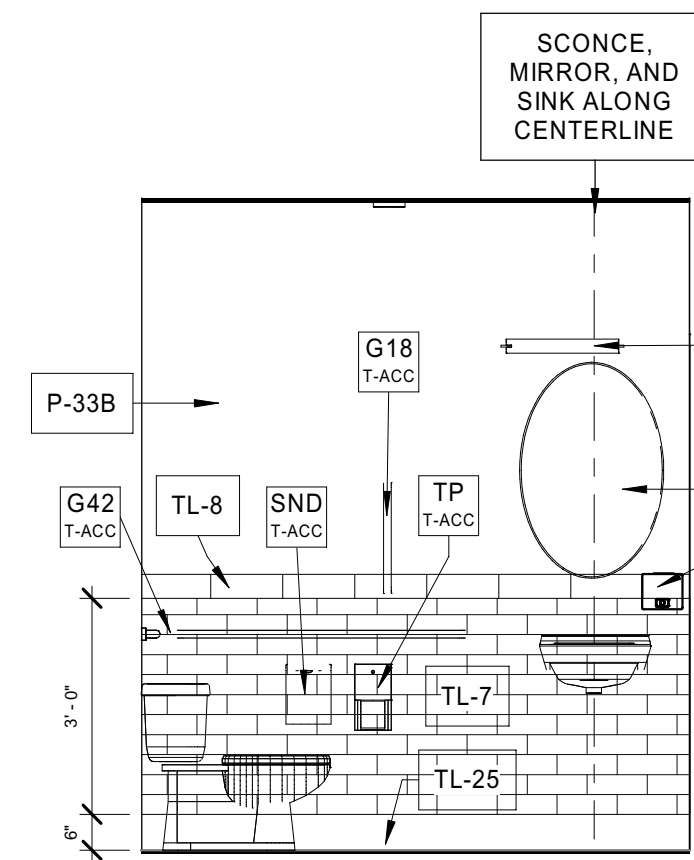
11 Interior Elevation UNISEX RR - 219 - S A5.12 3/8" = 1'-0"
