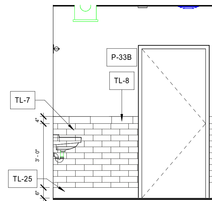
12 Interior Elevation UNISEX RR - 219 - W A5.12 3/8" = 1'-0"
