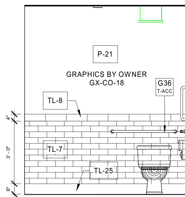
14 Interior Elevation UNISEX RR - 220 - E A5.12 3/8" = 1'-0"
