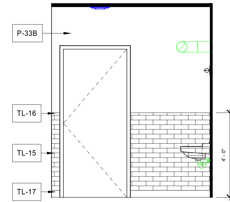
20 Interior Elevation UNISEX - 315 - W A5.12 3/8" = 1'-0"
