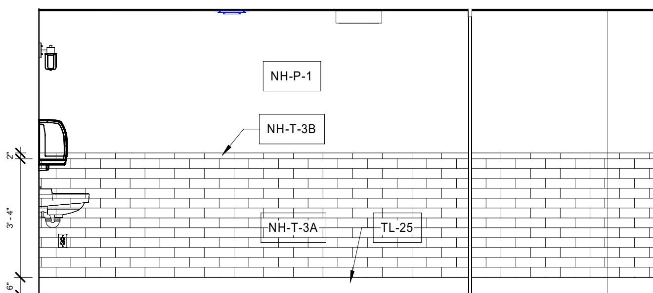
5 Interior Elevation WOMENS RR - 113 - N A5.12 3/8" = 1'-0"
