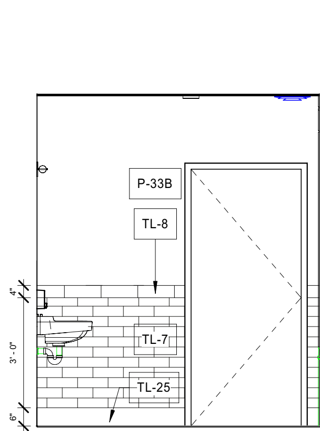
16 Interior Elevation UNISEX RR - 220 - W A5.12 3/8" = 1'-0"
