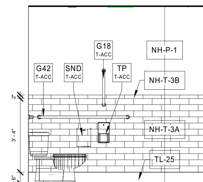
2 Interior Elevation MENS RR - 112 - E A5.12 3/8" = 1'-0"
